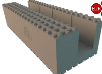
IsoteQ ® EXTRA Lintel Element
